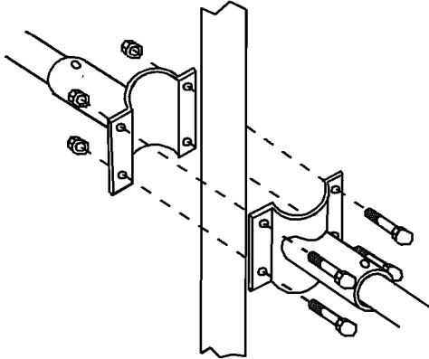
Vertical Mount Head to Head
