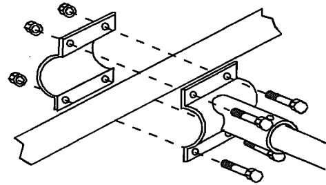
Horizontal Mount Single Row
